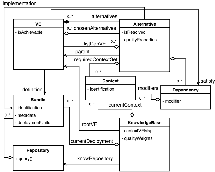
Fig. 7: GoalD-runtime metamodel
