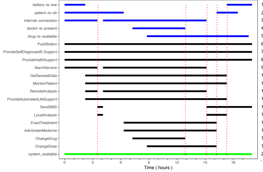
Fig. 9: Component Activation in GoalD
